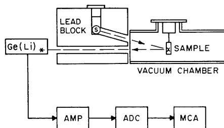
Fig. 2. Schematic diagram of a typical Compton scattering spectrometer using a \gamma -ray source.
