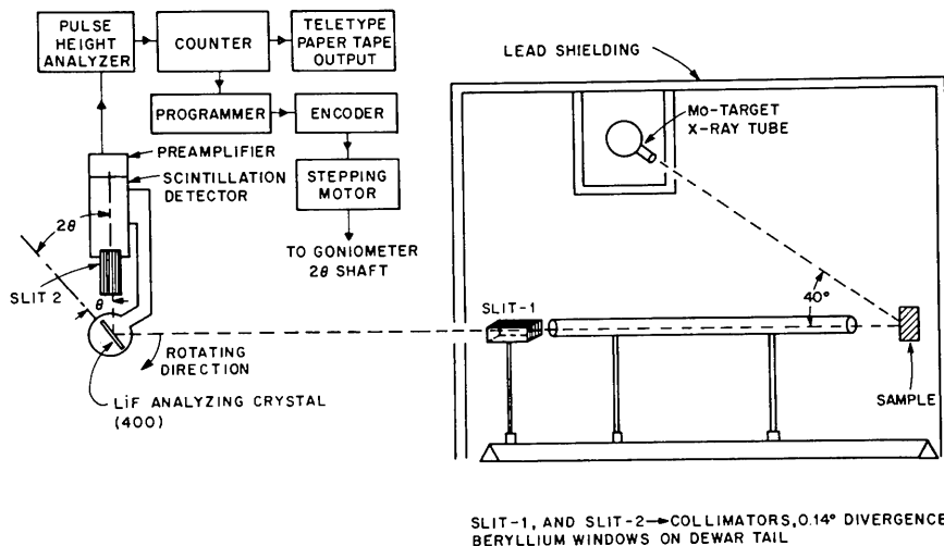
Fig. 1. Schematic diagram of a typical Compton scattering spectrometer using an X-ray source.
