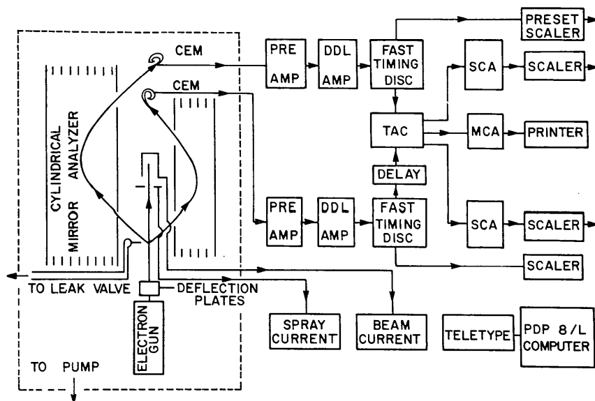
Fig. 5. Schematic diagram of a spectrometer used in ( e, 2e ) scattering.
