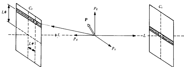
Fig. 6. Experimental arrangement for positron annihilation measurements.
