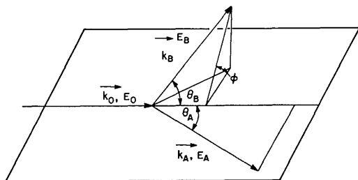
Fig. 4. Experimental arrangement for (e, 2e) measurements.
