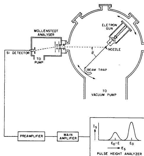
Fig. 3. Schematic diagram of a spectrometer used in high-energy electron Compton scattering.
