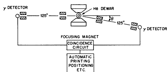
Fig. 7. Schematic diagram of a long-slit spectrometer used in positron annihilation measurements.
